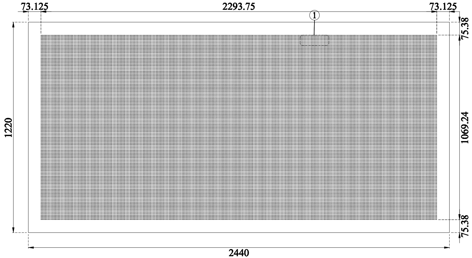
① Perforated Detail 3 x 3 mm @ 8.33 mm c/c
