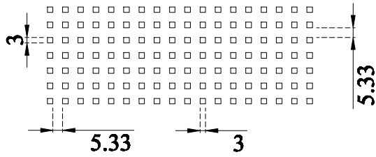
① Perforated Detail 3 x 3 mm @ 8.33 mm c/c
